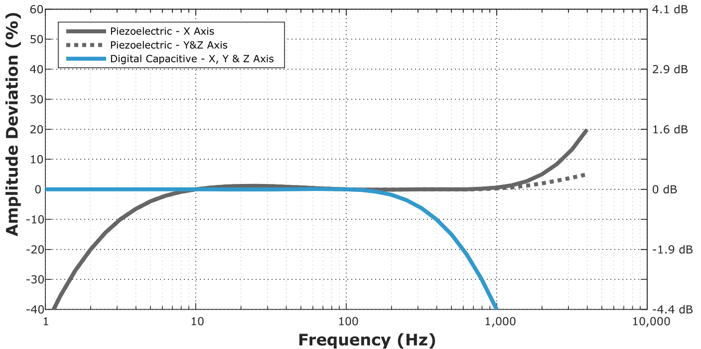
endaq S4-ExxxD40 Series Frequency Response
